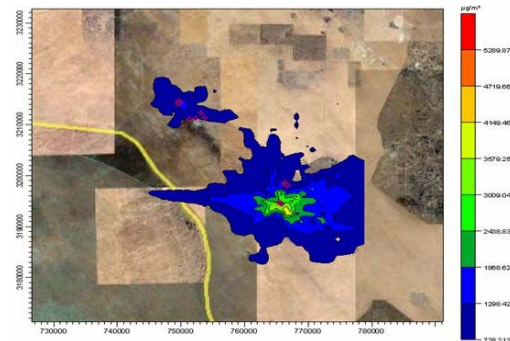
Fig. 7a Isoleths plot for the maximum hourly average ground level concentrations of non-methane hydrocarbons in \mu\text{g}/\text{m}^3
