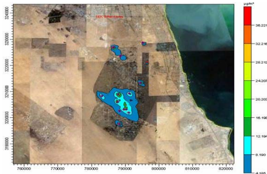
Fig. 3c Isoleths plot for the maximum annual average ground level concentrations of non-methane hydrocarbons in \mu\text{g}/\text{m}^3
