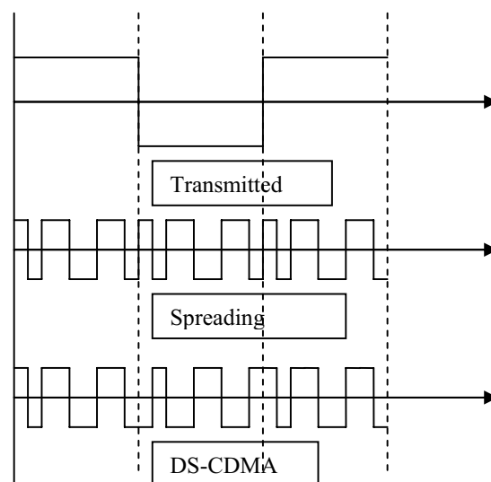
Fig. 1 DS-CDMA Modulation with spreading gain N=7
