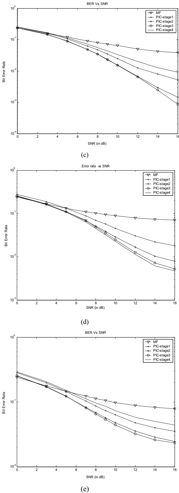
Fig. 5 BER Vs SNR for Multistage Detector with (a) 10- users, (b) 15- users, (c) 20- users, (d) 25- users and (e) 30- users
