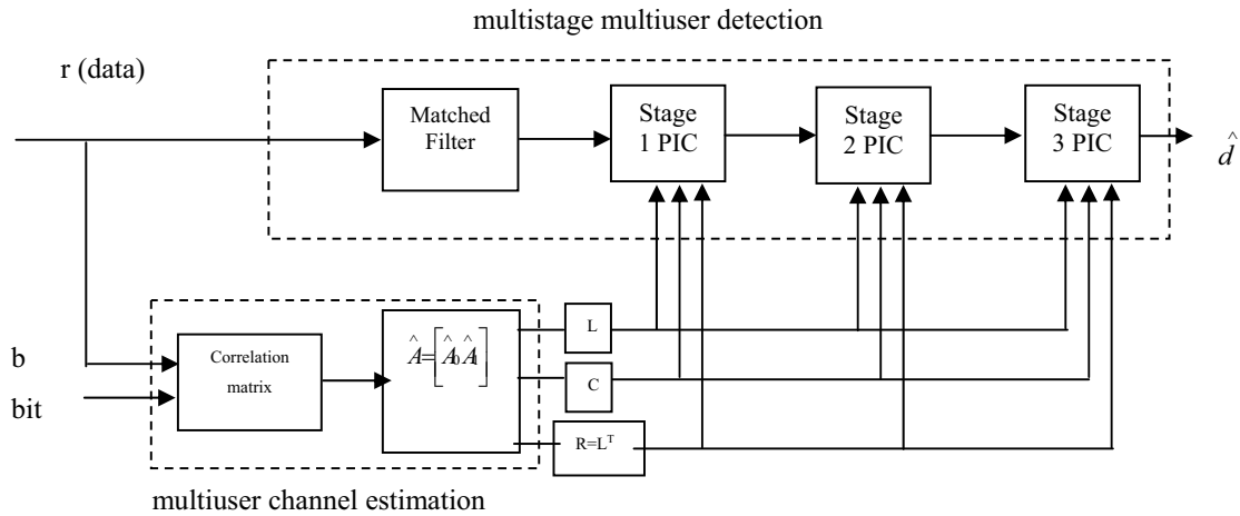
Fig. 4 The joint process of channel estimation and detection
