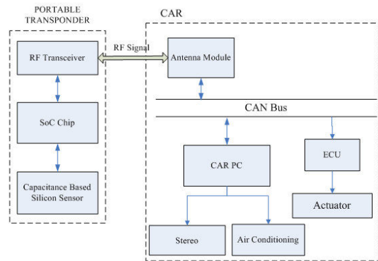
Fig. 3 Architecture of fingerprint identification keyless entry-system
