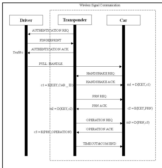
Fig. 5 Communication Sequence
