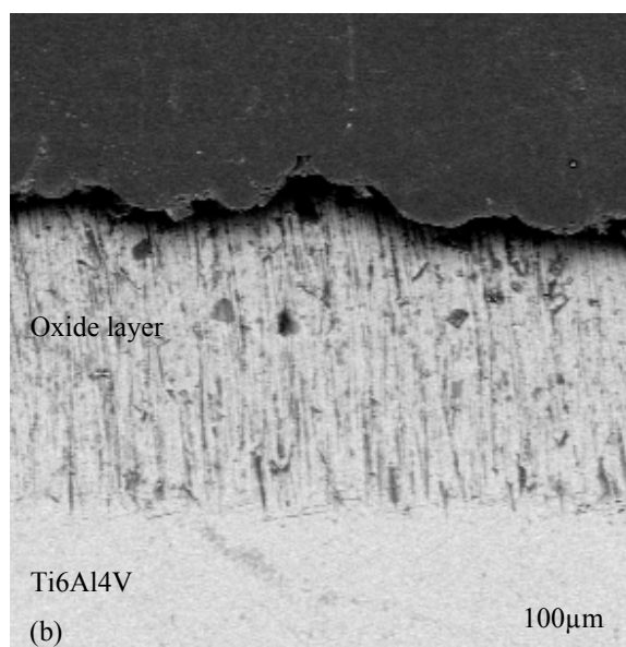
Fig. 1 SEM images showing cross-sectional view of the oxide layers: (a) anodized in 65 \pm 2 V and then oxidized at 950^\circ\text{C} for 5 h, (b) only thermally oxidized at 950^\circ\text{C} for 5h
