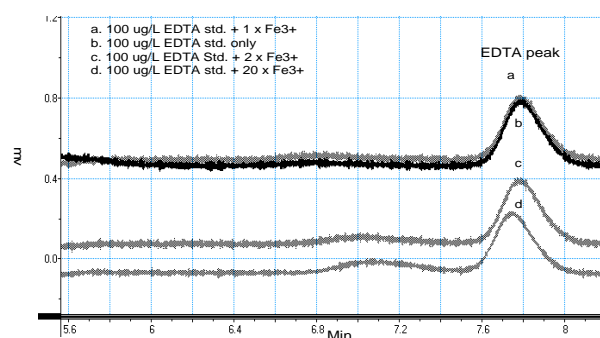
Fig. 5 Overlay of chromatograms by adding different levels of iron to a 100 \mu\text{g L}^{-1} EDTA standard solution. Conditions: Column, Hypersil \text{C}_{18} RP column (Phenomenex) of length 200 mm, diameter 4.6 mm and particle size 5 \mu\text{m} ; Mobile phase, 2% MeOH, 15 mM TBABr in pH 3.3 sodium formate/formic acid buffer solution; sample loop, 50 \mu\text{L} ; Flow rate, 0.9 \text{ mL min}^{-1} ; Wavelength, 265 nm
