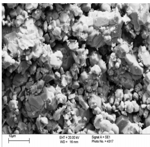
Fig. 4 SEM micrograph of the oxide after oxidation at 1000° C
