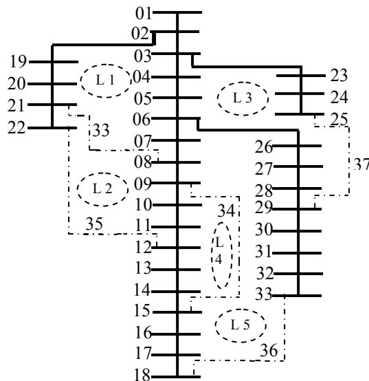
Fig. 5 33-Bus radial distribution system with loops
