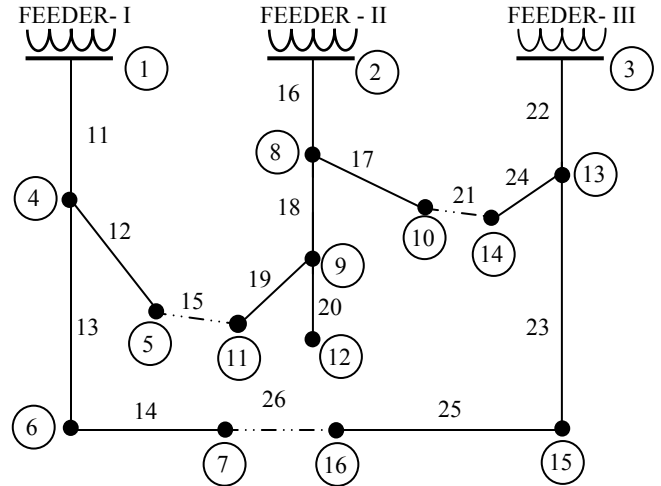
Fig. 3 Three-feeder, 14 bus distribution system
