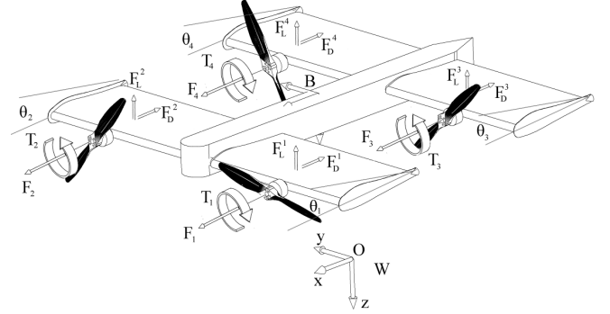
Fig. 3. Aerial Vehicle in Horizontal Flight Configuration
