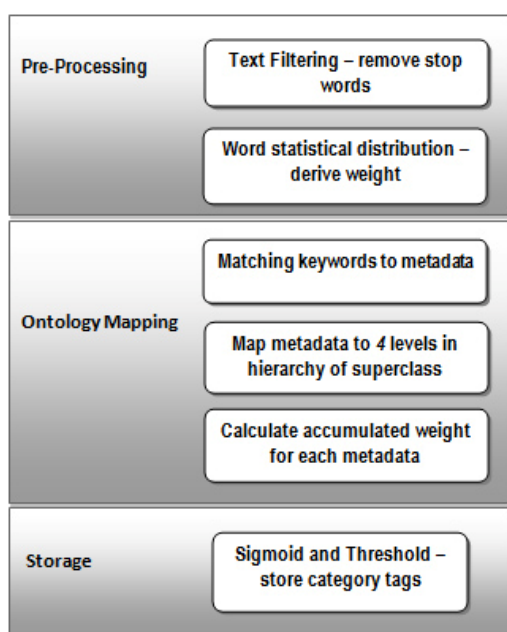
Fig. 2 Processes involved in the ontology mapping phase
