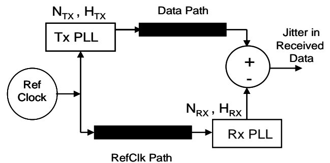
Fig. 1 Generic model of jitter propagation commonly found in high speed data link architecture
