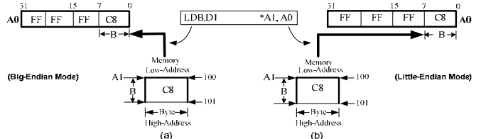
Fig. 15 Example of reading a byte (B) from memory in big and little endian mode
