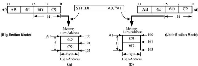
Fig. 11 Example of storing a half-word(H) in the memory in big and little endian mode
