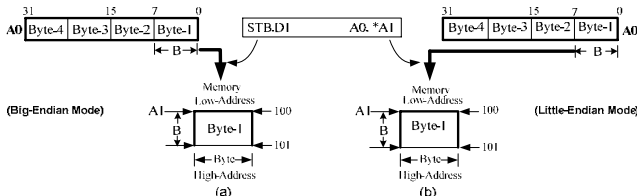
Fig. 9 Storing a byte (B) of data in the memory in big and little endian mode
