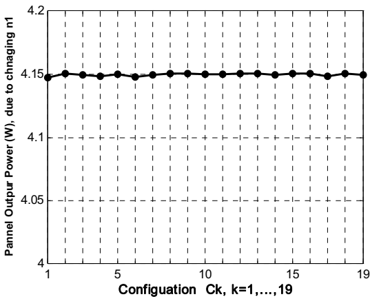
Fig. 10 Variation of panel output power for all layouts, U_1 to U_{19} due to changing n_1 from 0.9 to 1.0 for a temperature of 27°C
