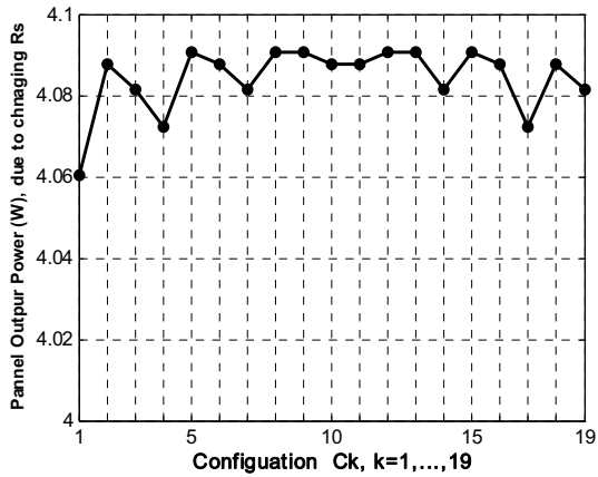
Fig. 11 Variation of panel output power for all layouts, U_1 to U_{19} due to changing of series resistance R_s from 0.01Ω to 0.05Ω for a temperature of 27°C
