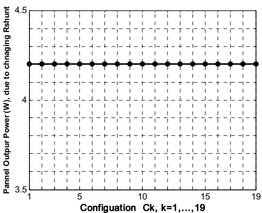
Fig. 12 Variation of panel output power for all layouts, U_1 to U_{19} due to changing shunt resistance R_{SH} from 100Ω to 300Ω for a temperature of 27°C.
