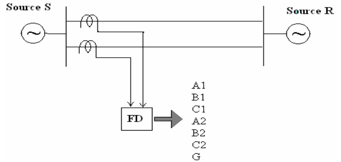
Fig. 1 power System under Study
