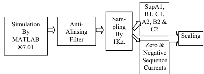
Fig. 3 training patterns generation process
