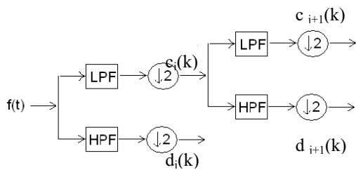
Fig. 1 Decomposition Tree
