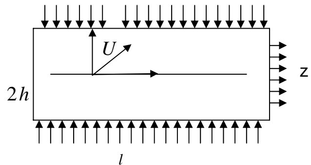
Fig. 5 Physical and geometric models of rectangular chamber
