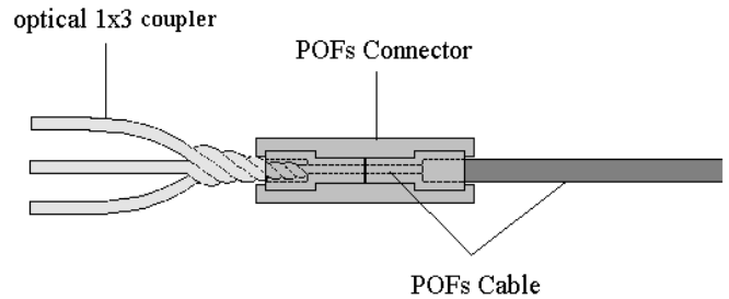
Figure 7. Connection between optical 1x3 coupler with 1 mm POF cable
