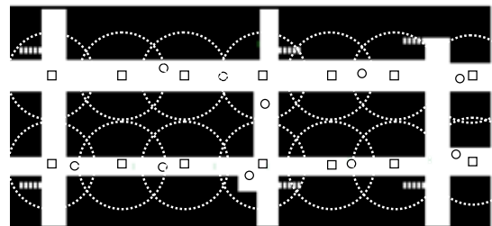
(c) The interaction of active RFID reader and pedestrian agent
