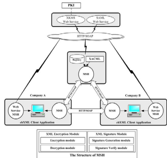
Fig. 6 Architecture of the ebXML test software
