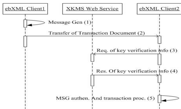
Fig. 5 Sequence Diagram – Scenario 2
