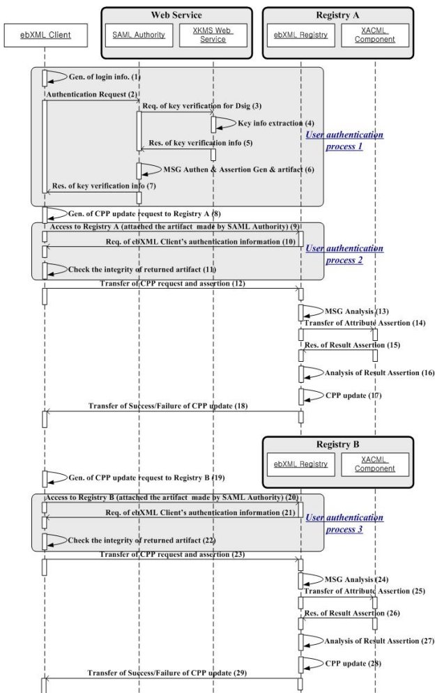
Fig. 4 Sequence Diagram – Scenario 1
