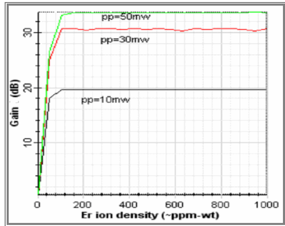
Fig. 5 Gain at different Er^{+3} ion density after optimization relative to each optimum length at pumping powers 10, 30 and 50mw
