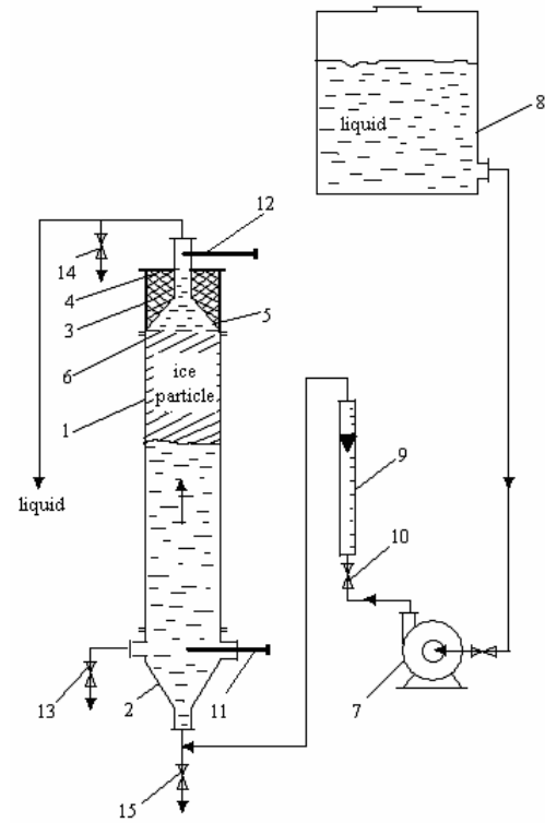
Fig. 1 Experimental installation (1- column, 2 - conical section, 3 – cylindrical section, 4 – lid, 5 – funnel, 6 – sieve, 7 – pump, 8 – reservoir, 9 – rotameter, 10, 13 and 14 – valves, 12 – thermocouples).
