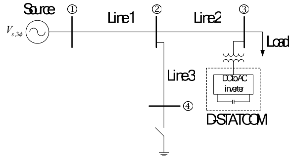
Fig. 6 Simplified 4-bus test system
