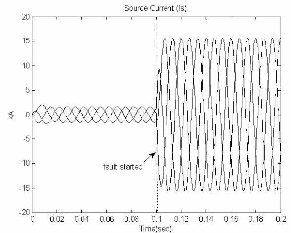
Fig. 12 Source currents of the D-STATCOM case
