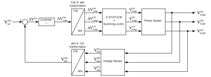
Fig. 3 Complete block diagram of voltage regulation scheme
