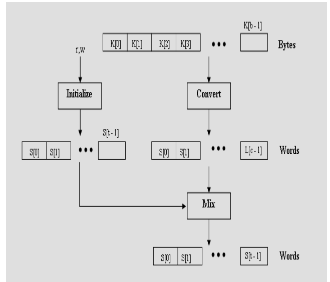
Fig. 15. RC5 Key expansion[8]
