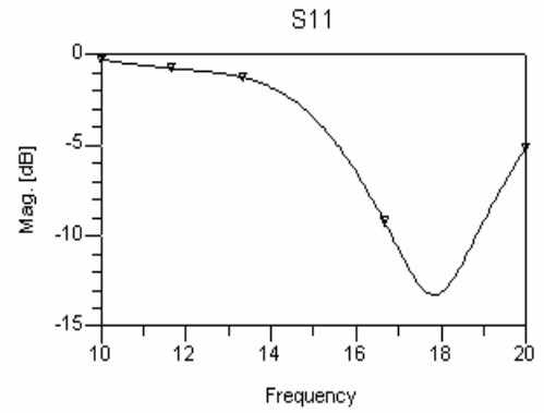
Fig. 6 The input reflection coefficient of the circular patch microstrip array antenna
