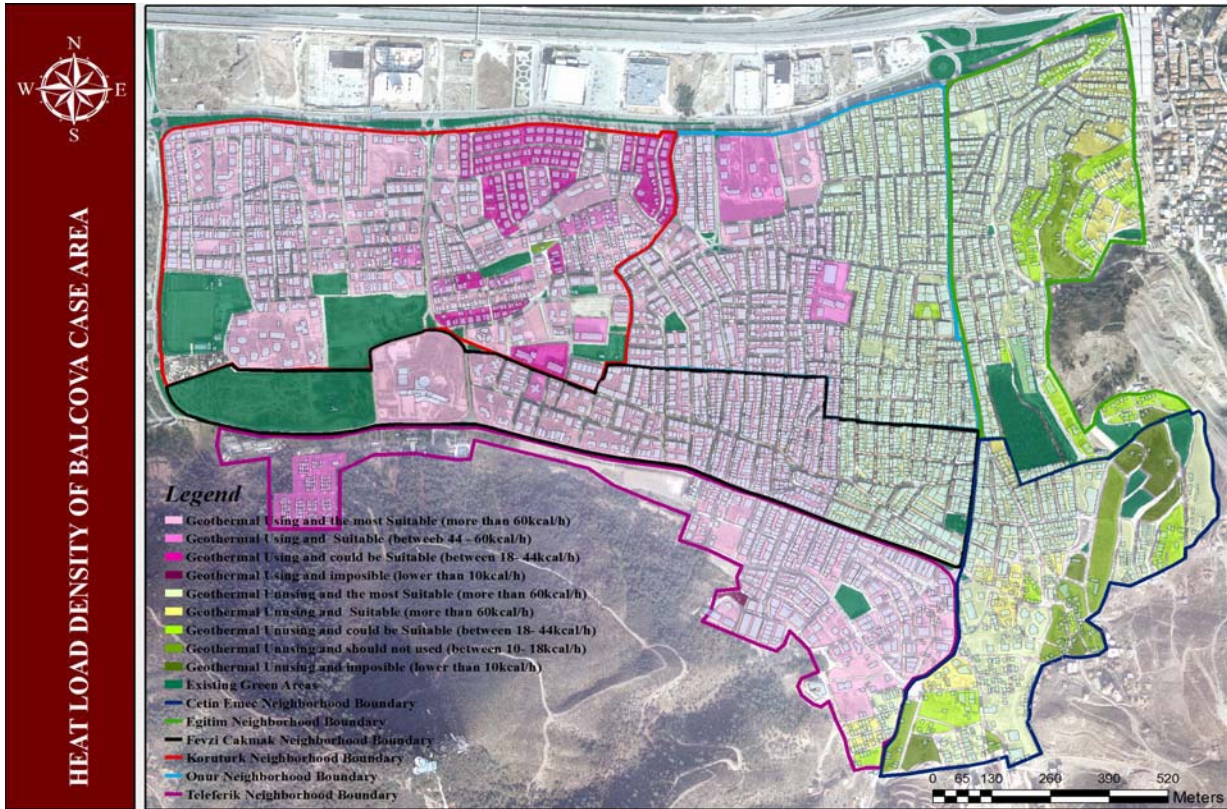
App. I.c. Existing Heat Load Density
