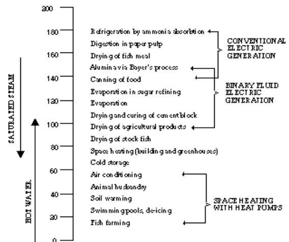
Fig. 2. Lindal Diagram
