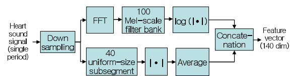
Fig. 4 Feature extraction for ELM-based classifier.
