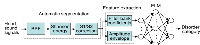
Fig. 1 The ELM-based heart sound classification system.
