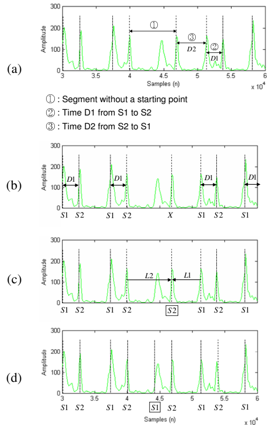
Fig. 3 Procedure of starting-point correction. (a) Inter-pulse duration has 3 different kinds. (b) Starting points of S1/S2 pulses are labeled. (c) Unlabeled pulses are resolved. (d) Missing or incorrect pulses are corrected.
