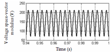
Fig. 11 Evolution of the voltage vector modulus
