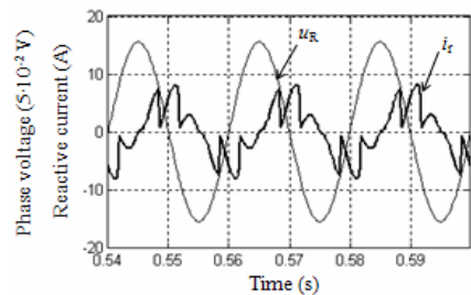
Fig. 5 Phase voltage and reactive current defined by (6)
