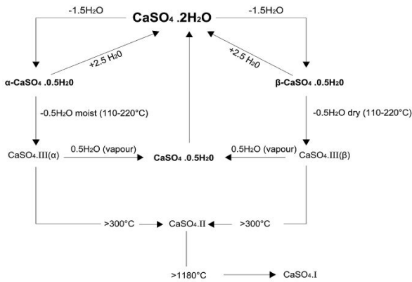
Fig. 1 Different modifications of \text{CaSO}_4 \cdot x\text{H}_2\text{O} ( x = 0.0-2.0 ).
