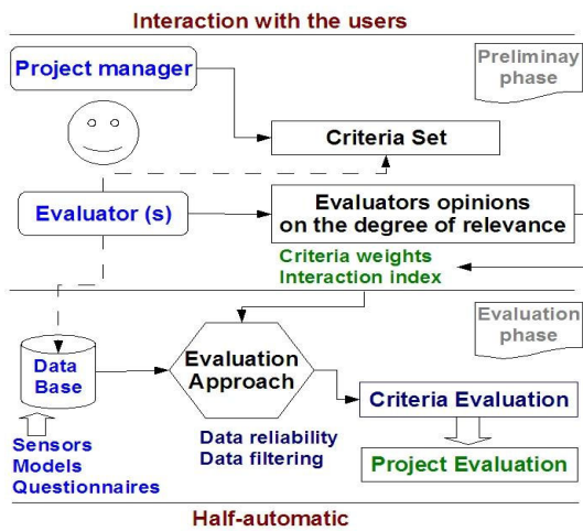
Fig. 1 Evaluation approach
