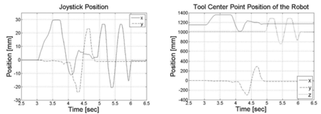
Fig. 8 Translational mapping: joystick position (left) and TCP position of the robot (right)
