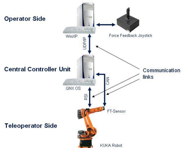
Fig. 2 System architecture
