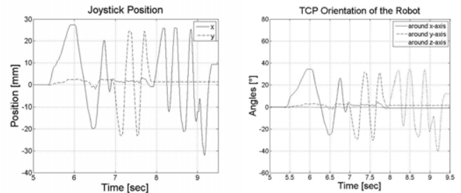
Fig. 9 Rotational mapping: joystick position (left) and TCP orientation of the robot (right)
