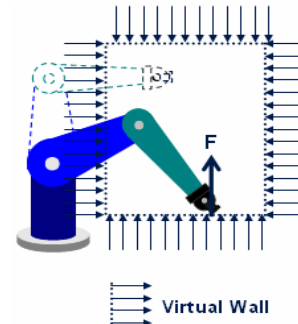
Fig. 4 Workspace limits
