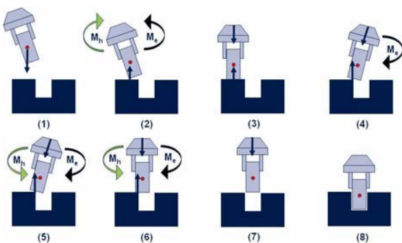
Fig. 1 Peg-in-hole assembly task. M_e and M_h are the error related and
