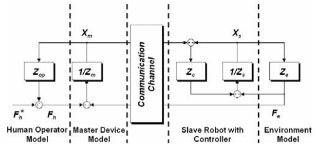
Fig. 3 A classical position/force bilateral control scheme of a teleoperation system [10]
