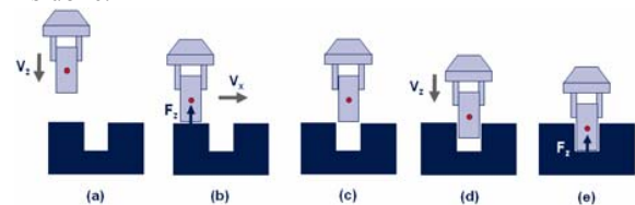
Fig. 5 Simulation scenario
