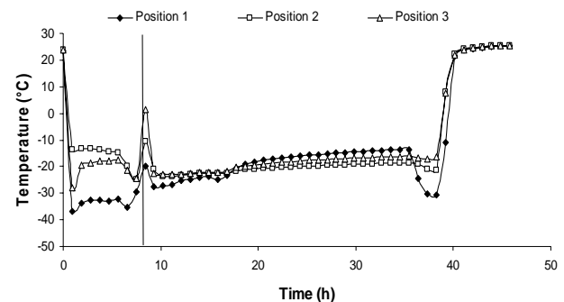
Fig. 2 Temperature change at level 1 inside the grain bin during trial 1
