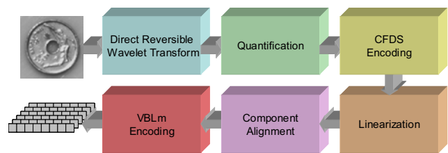
Fig. 1 General description of the compression system.
