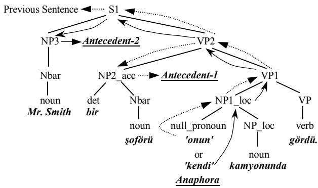
Fig. 3. The illustration of the parse tree of sentence (4) and the algorithm working on it.
