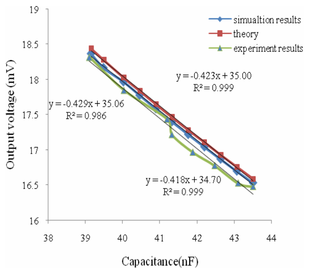
Fig. 6 Output voltage versus capacitance at 3 kHz
