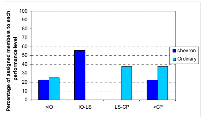
Fig. 7 knee element performance levels of 7-storeys frames
