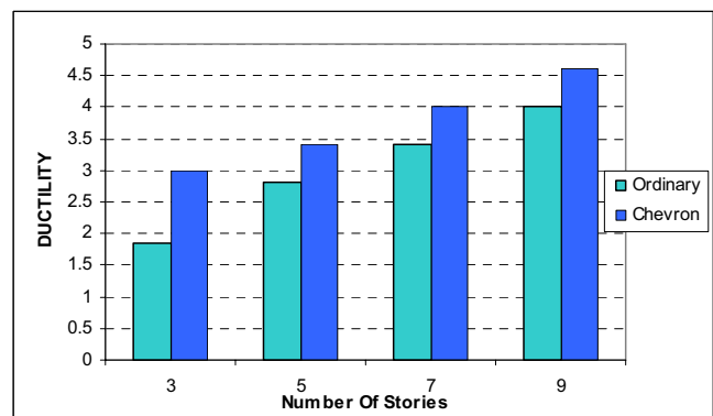
Fig. 9 Comparison of ductility factors in frames
