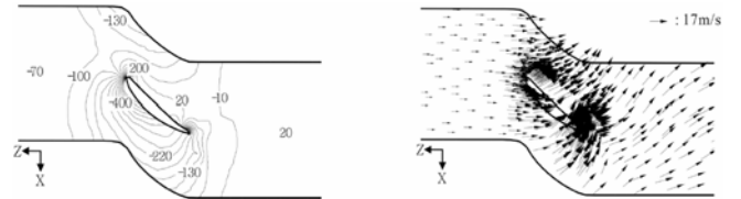
(a) Distribution of static pressure [Pa] (b) Distribution of absolute velocity vectors Fig. 8 Numerical results on the mid-span plane of 64° pitch angle of impeller blade
