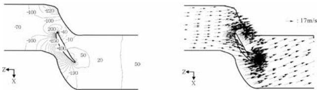
(a) Distribution of static pressure [Pa] (b) Distribution of absolute velocity vectors Fig. 6 Numerical results on the mid-span plane of 44° pitch angle of impeller blade
