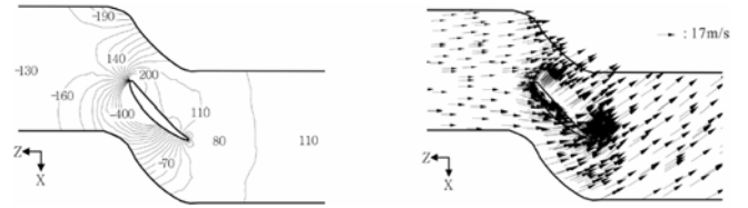
(a) Distribution of static pressure [Pa] (b) Distribution of absolute velocity vectors Fig. 7 Numerical results on the mid-span plane of 59° pitch angle of impeller blade
