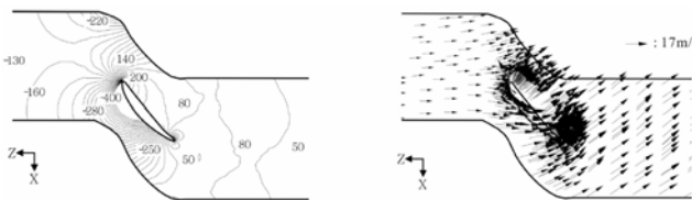
(a) Distribution of static pressure [Pa] (b) Distribution of absolute velocity vectors Fig. 5 Numerical results on the mid-span plane of 54° pitch angle of impeller blade
