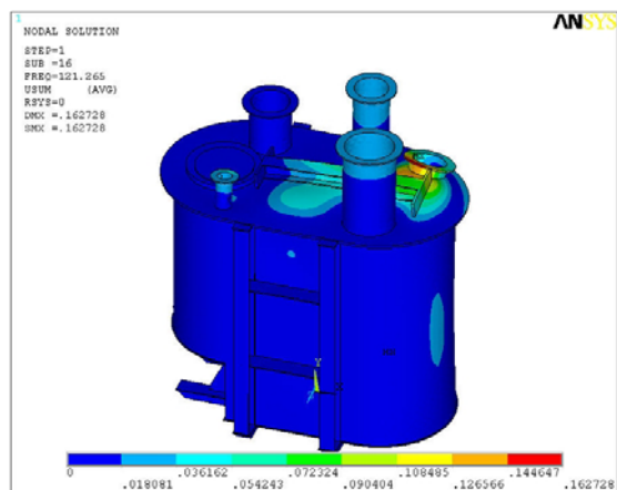
Fig. 4 16 th resonance (121.3 Hz)
