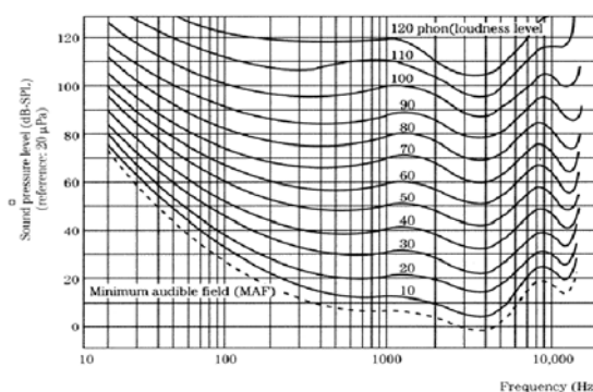
Fig. 1 Loudness curve
