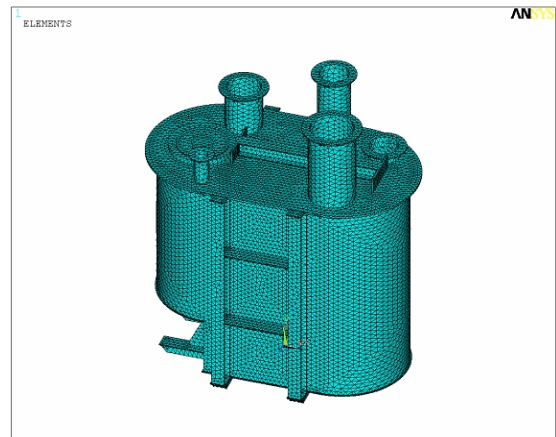
Fig. 3 Mesh shape
