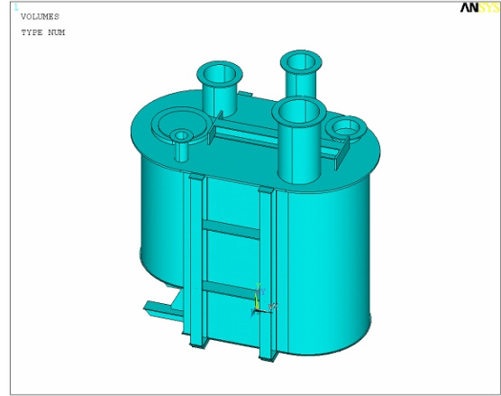
Fig. 2 Finite element model
