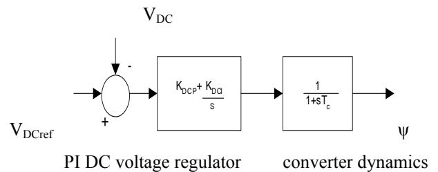
Fig. 5 STATCOM dynamic model of DC –Voltage regulator with the PWM Converter
