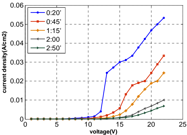
Fig. 3 J-V characteristic of OLED with structure of ITO/PEDOT:PSS/PFO/Al during the time after fabrication which has been measured in atmosphere condition
