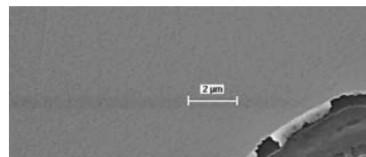
Fig. 6 SEM image of defected ITO of Fig. 5 in larger scale
