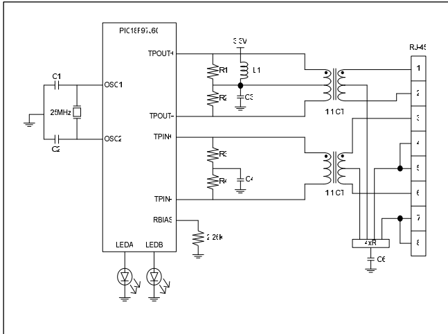
Fig. 4 External components for Ethernet
