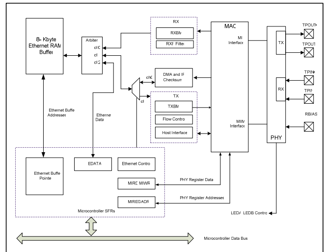
Fig. 3 Block diagram for Ethernet module system
