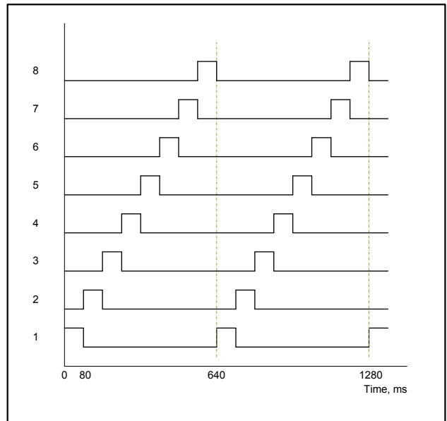
Fig. 5 Working Condition
