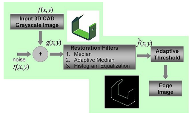
Fig. 2. Preprocessing flow.
