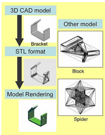
Fig. 1. Generation flow.
