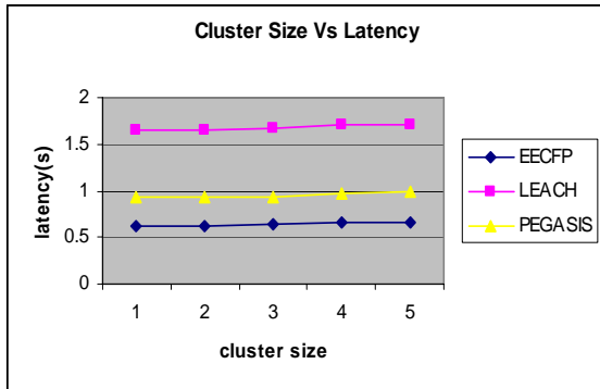
Fig. 6 Cluster Size Vs Latency
