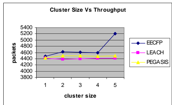
Fig. 5 Cluster Size Vs Throughput
