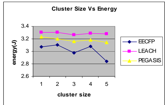
Fig 4 Cluster Size Vs Energy
