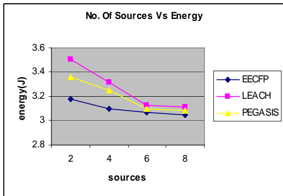
Fig. 7 Sources Vs Energy
