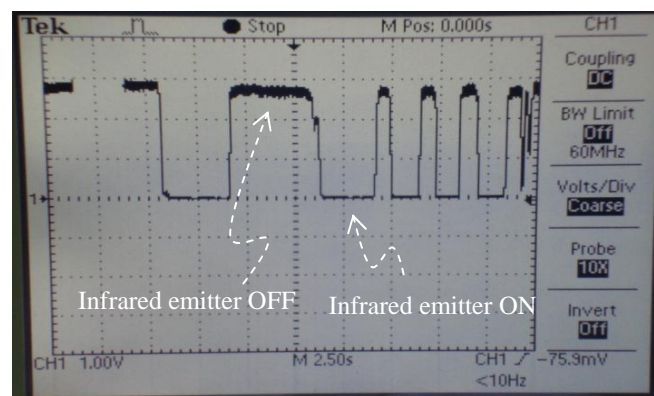
Fig. 12 Sensing ability of the MRV
