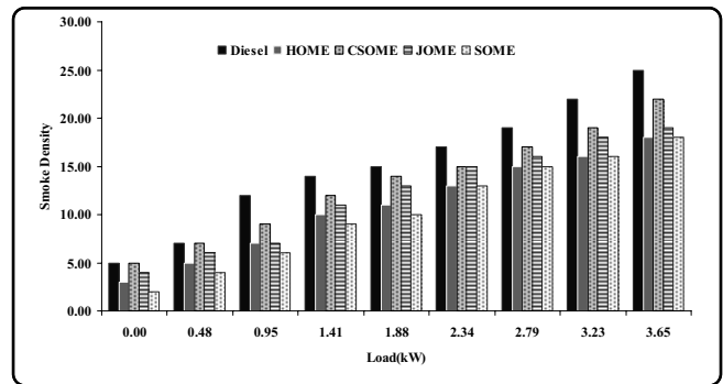
Fig. 5 Variation of smoke density (%) with applied load
