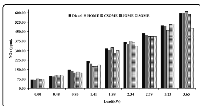
Fig. 8 Variation of \text{NO}_x emission with applied load
