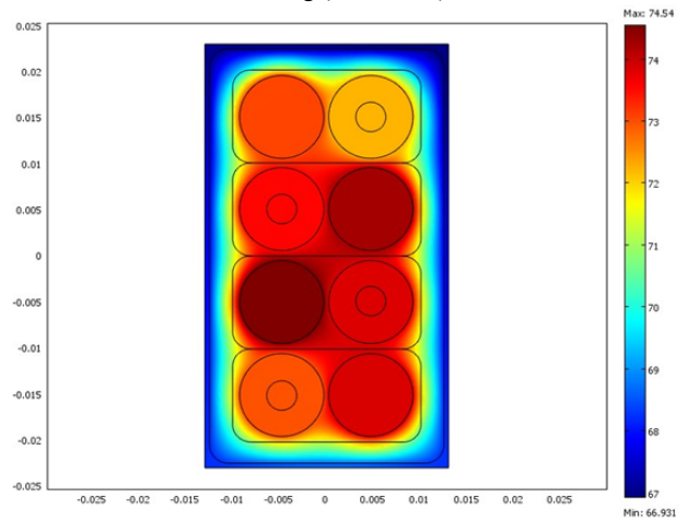
Fig. 5.b Thermal distribution of circular wiring (°C) - direct cooling with water (structure 4)
