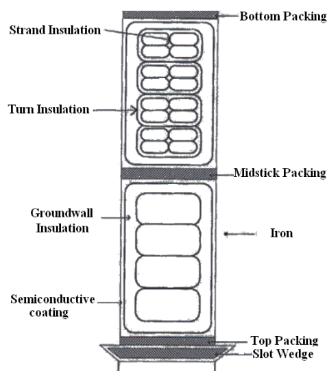
Fig. 1 Cross section of slots containing form-wound multi-turn coils
