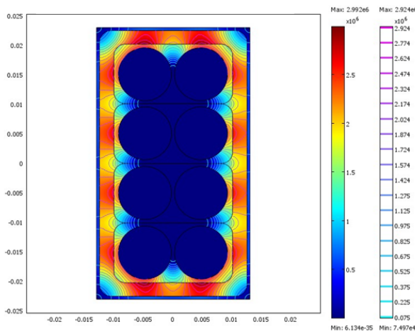
Fig. 4 Electrical field distribution of circular winding (V/m)
