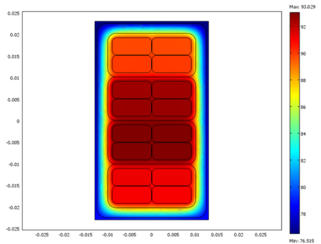
Fig. 3.a Thermal distribution of rectangular winding (°C) -natural cooling (structure 1)
