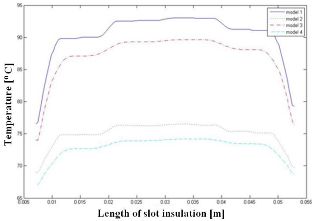
Fig. 6 Thermal distribution comparison in 4 structures studied
