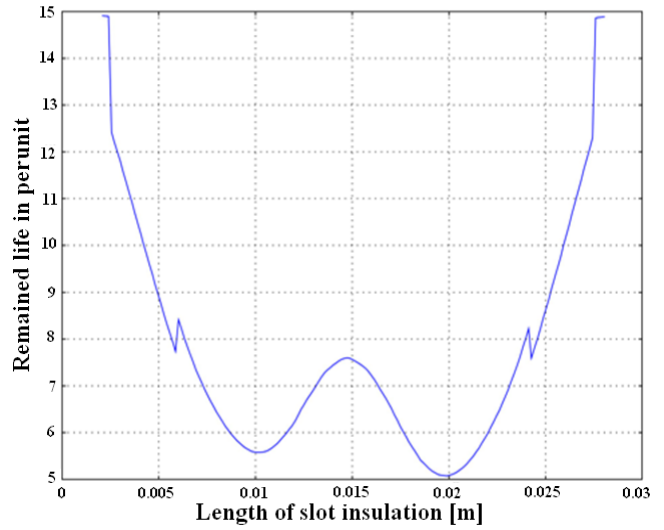
Fig. 7.b Remained life of insulation part of circular wiring - with cooler
