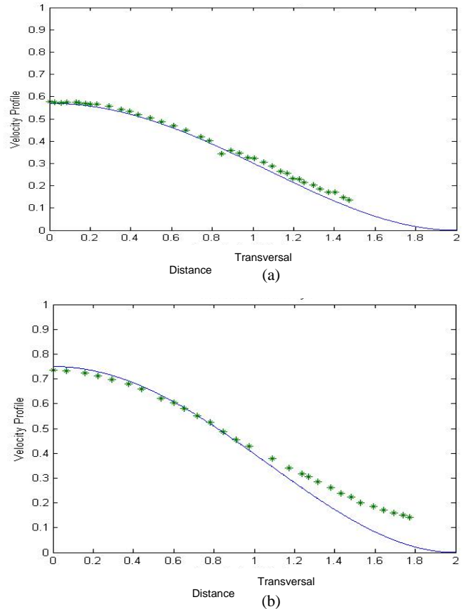
Fig. 2 Velocity profile in transverse coordinate performed by analytical solution (solid line) and the experimental data (points) for laminar free jet for (a) Re 5 and (b) Re 20 [13]
