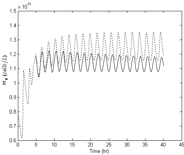
Fig. 11 Transient response of total cell number per unit volume. S_f/S pair loop is open (dash line), S_f/S pair loop is closed using a GLC (line)
