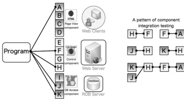
Fig. 12. A component-based Web programming
