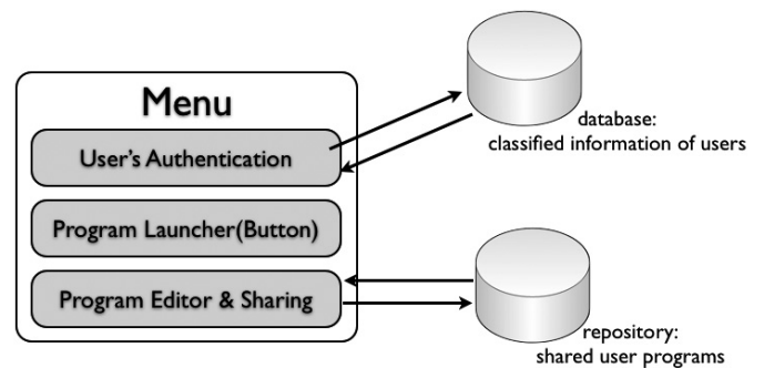
Fig. 7. Menu:feature manager
