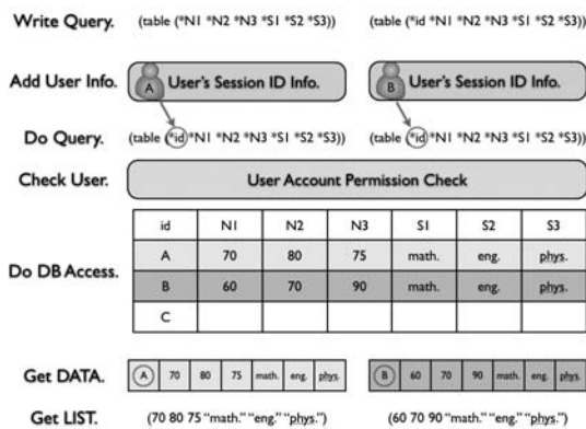
Fig. 8. User Authentication
