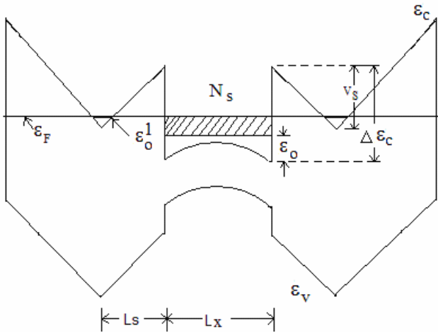
Fig. 4. A simplified Energy band diagram of a delta doped GaAs/AlGaAs Quantum well
