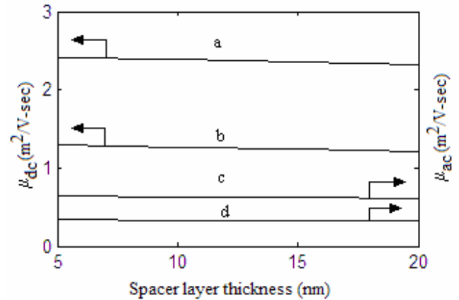
Fig. 7. Plot of \mu_{ac} and \mu_{dc} with spacer layer thickness L_s for L_x=10 \text{ nm} , N_i=6 \times 10^{21} \text{ m}^{-3} and n^{2D}=1 \times 10^{16} \text{ m}^{-2} . Curves a and c show the results for delta doped QW and curves b and d are for conventional homogeneously doped QW.
