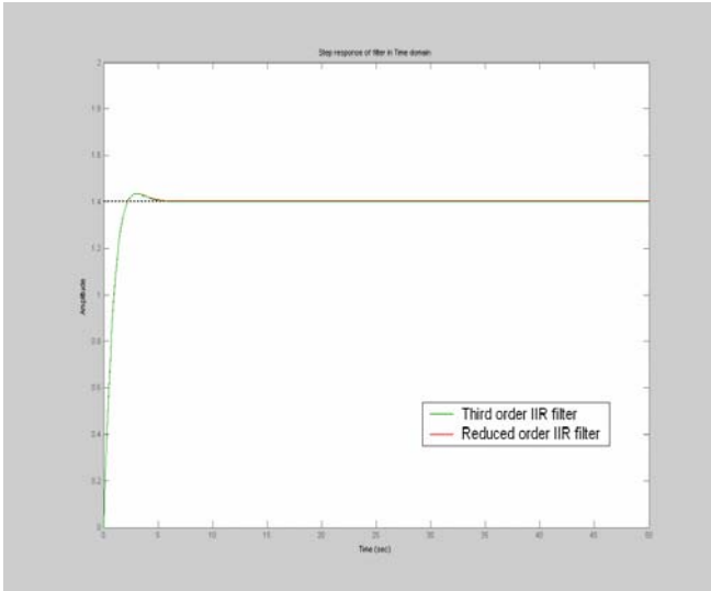
Fig.2 Comparison of Step responses
