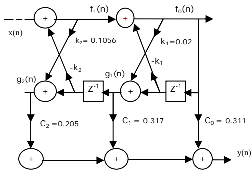
Fig.6 Structure of Reduced order Lattice-ladder IIR filter
