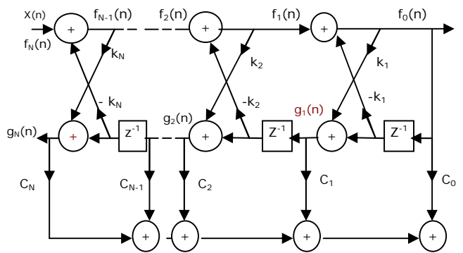
Fig.1 Structure of Lattice-ladder IIR filter of N^{\text{th}} order
