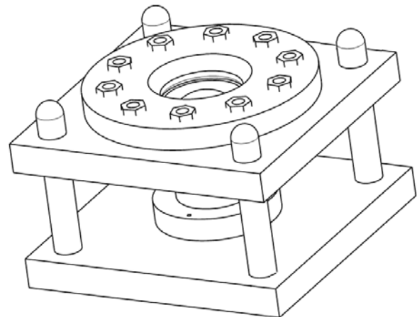
(a) 3D drawing of deep drawing die
