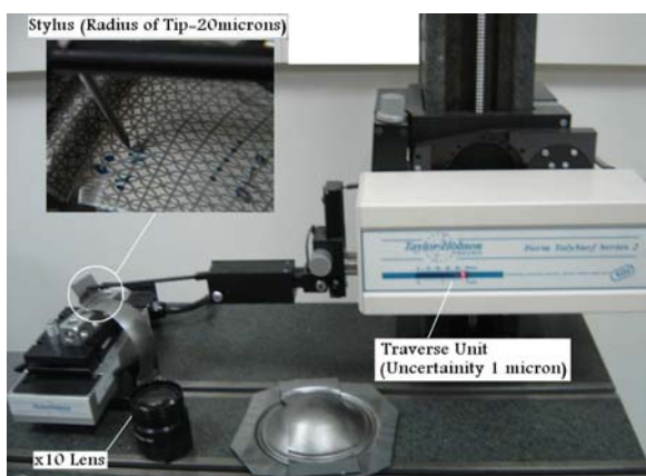
Fig. 5 Measurement of circle diameters by Form Talysurf
