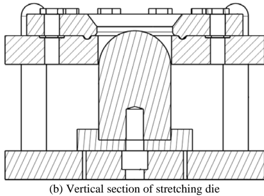
Fig. 1 Drawing of stretching die
